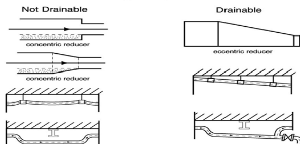
Fig. 12. Non-drainable and drainable designs of pipelines
